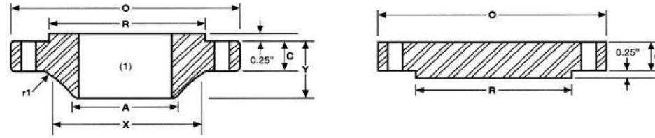
Weld Neck
