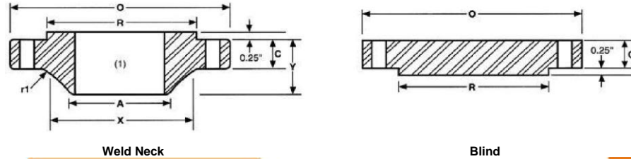
Weld Neck
